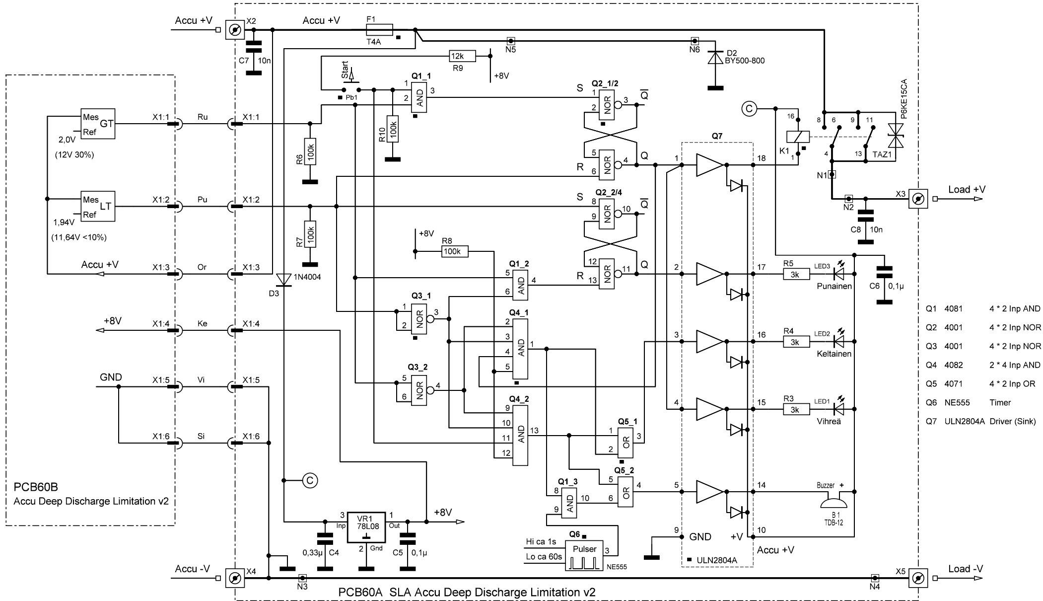
Pb Accu Deep Discharge Limitation v2 PCB60A_A Logic Section Connection Diagram
