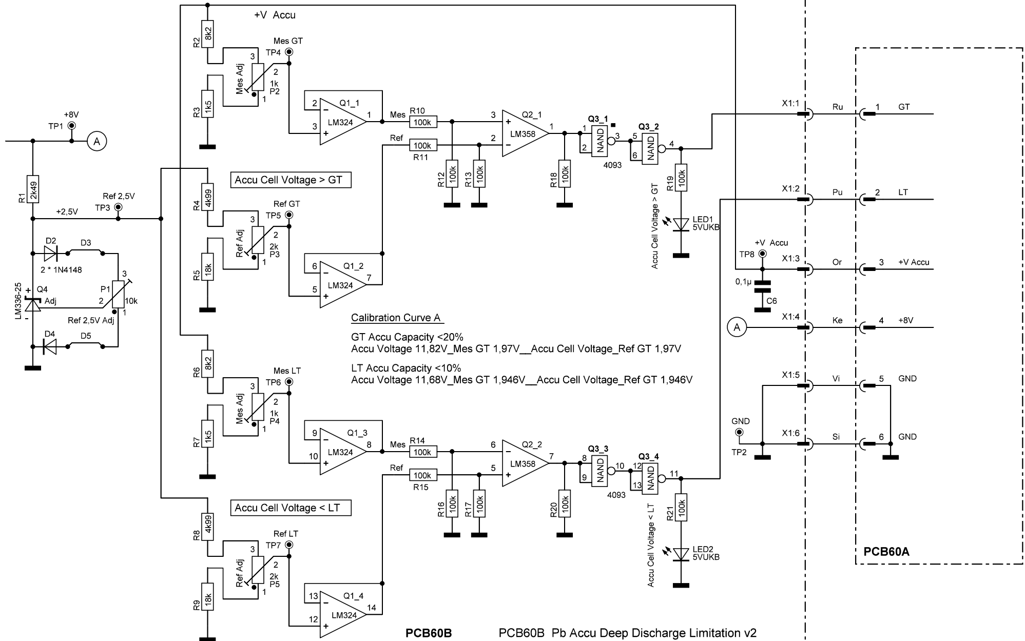
Pb Accu Deep Discharge Limitation v2 PCB60B_A Analogue Section Connection Diagram
